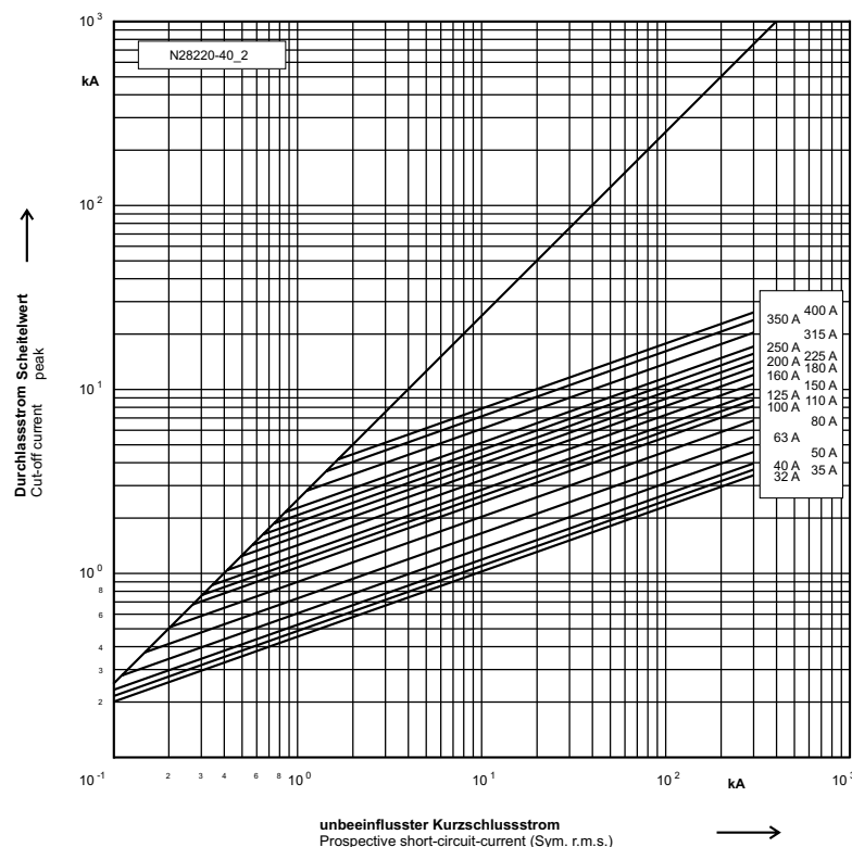
Durchlass-Strom Cut-off current
