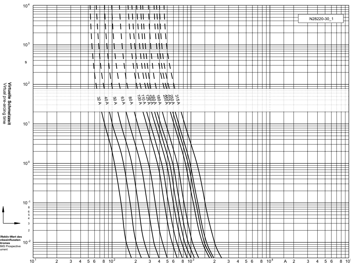
Zeit/Strom-Kennlinien Time-current characteristics
